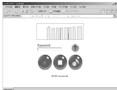
Figure 3. Client Interface.
